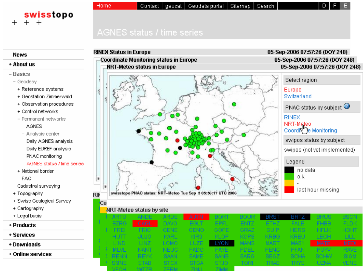
Fig. 3: Monitoring page of swisstopo for the availability of NRT ZTD-estimates. ( http://www.swisstopo.ch/en/basics/geo/permnetworks/pnac/timeseries/timeseries_nrt_meteo_europe ).
