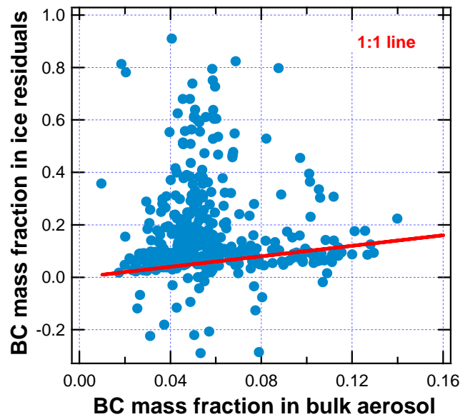
Figure 3. Simultaneously measured BC mass fraction for ice residuals and for the bulk aerosol. The BC mass fraction is defined as the ratio of the particle BC mass concentration to total aerosol mass concentration.
