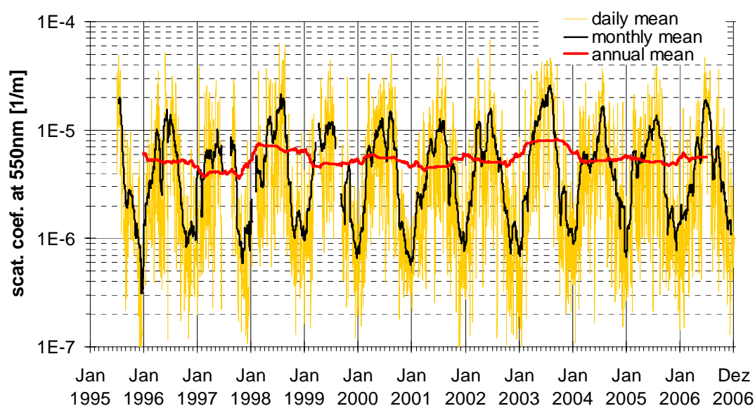
Figure 1. Long-term measurements of the light scattering coefficient (at 550 nm).
