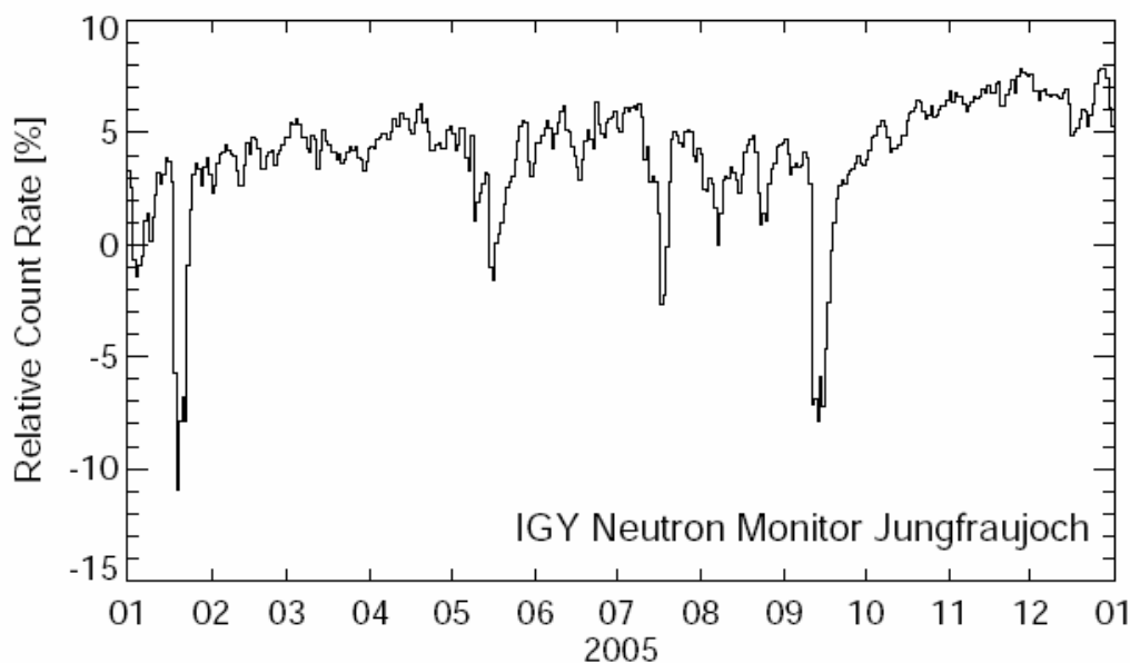
Figure 1: Relative pressure corrected daily counting rates of the IGY NM at Jungfraujoch for 2005.
