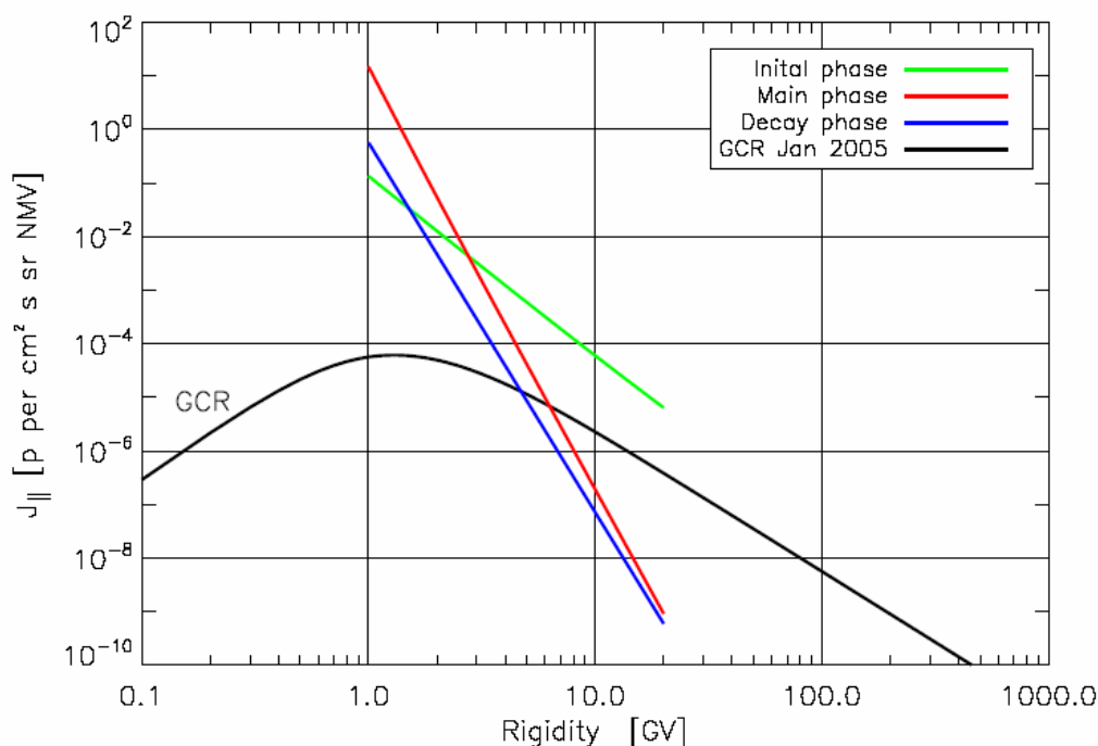
Figure 5: Solar cosmic ray ( J_{\parallel} ) and galactic cosmic ray (GCR) spectra near Earth during the giant solar particle event on January 20, 2005.
