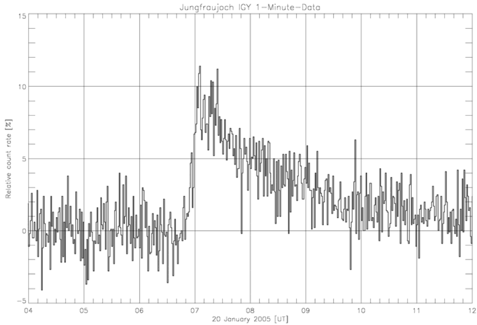
Figure 3: Relative pressure corrected 1-minute counting rates of the IGY NM at Jungfrauoch for January 20, 2005, 0400-1200 UT.
