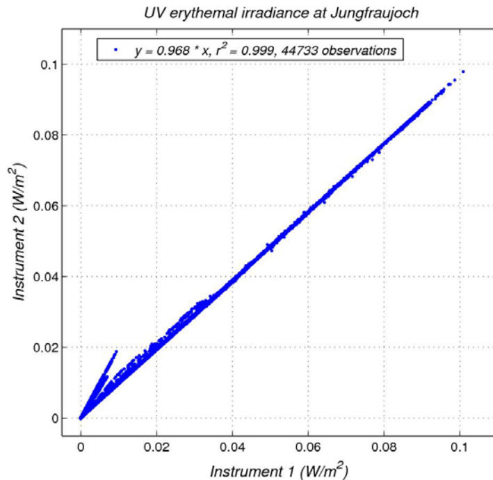
Figure 2. Comparisons of concurrent erythemally-weighted irradiance measurements by two collocated biometers at Jungfraujoch (26/10/2005-31/12/2005).
