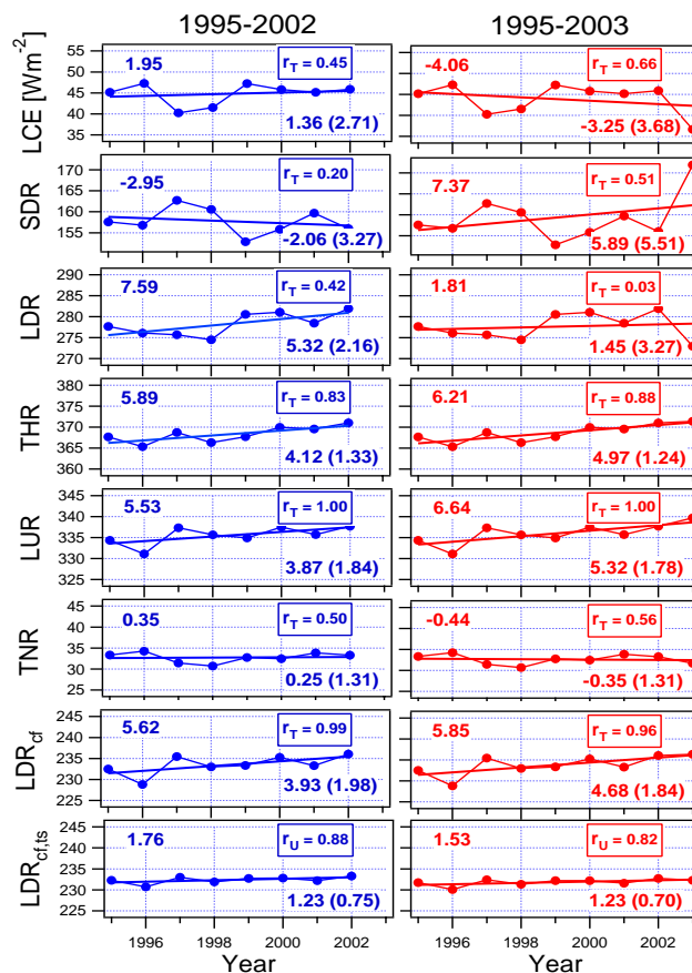
Figure 1: Annual means of individual radiative fluxes averaged over the six ASRB stations shown for the periods 1995-2002 (left) and 1995-2003 (right). Descending in the rows: longwave cloud effect (LCE), shortwave downward radiation (SDR), longwave downward radiation (LDR), total heating radiation (THR), longwave upward radiation (LUR) also corresponds to surface temperature, total net radiation (TNR), cloud-free longwave downward radiation ( LDR_{cf} ), temperature subtracted cloud-free longwave downward radiation ( LDR_{cf,ts} ). Numbers in framed boxes indicate the correlation index to temperature for the first 7 fluxes and to absolute humidity for LDR_{cf,ts} .
