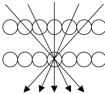
Figure 2: Cross-section in the north-south direction of the bottom proportional counters illustrating the principle for determining directional information. For details see the text.
