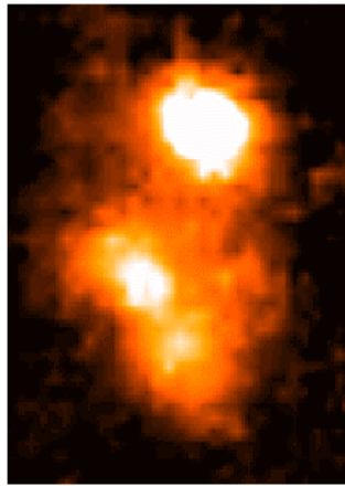
Fig. 1: mid-IR image of a cluster of forming stars in the Orion nebula. The field-of-view is 24"x29" with a pixel of 0.77". The total integration time is 2.5 min. The image was obtained by chopping between the object and the nearby sky at a frequency of 3 Hz
