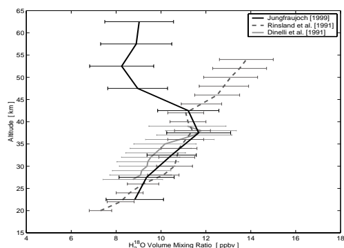
Comparison of vmr for \text{H}_2\text{O}^{18} deduced from EMCOR with data from ATMOS, an IR solar occultation experiment, and data from a balloon borne Fourier transform instrument
