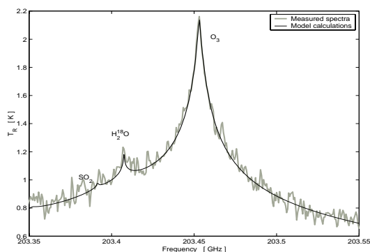
Spectra of \text{O}_3 and \text{H}_2\text{O}^{18} measured with EMCOR from Jungfraujoch with corresponding synthetic spectrum based on the retrieved profile
